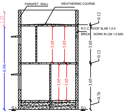
Section on-"AA"
