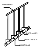
STAIR CASE DETAILS
