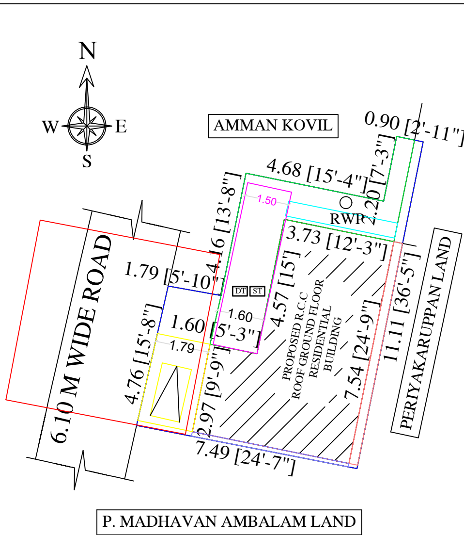
SITE PLAN
