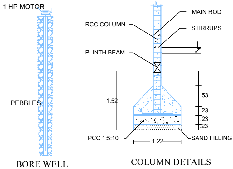
COLUMN DETAILS
