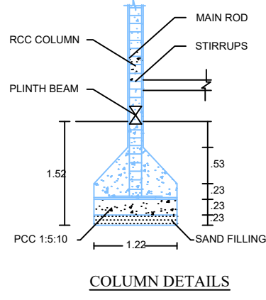
COLUMN DETAILS
