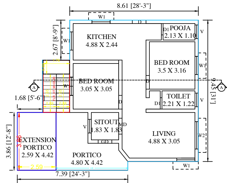
ADDITIONAL GROUND FLOOR PLAN
