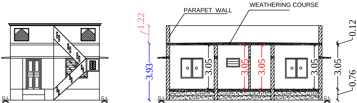
Front Elevation
