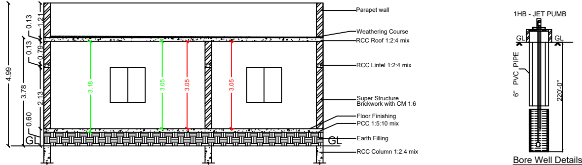
SECTION ON "VR"
