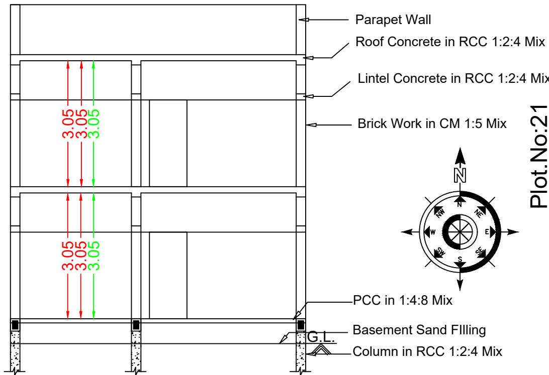
Section RR
