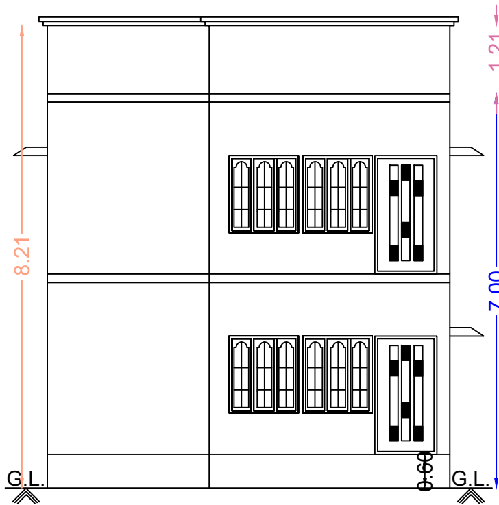
Front Elevation
