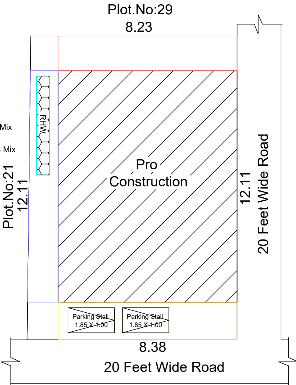
Site Plan
