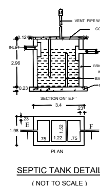
SEPTIC TANK DETAILS (NOT TO SCALE)
