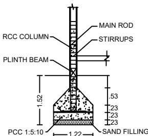
COLUMN DETAILS
