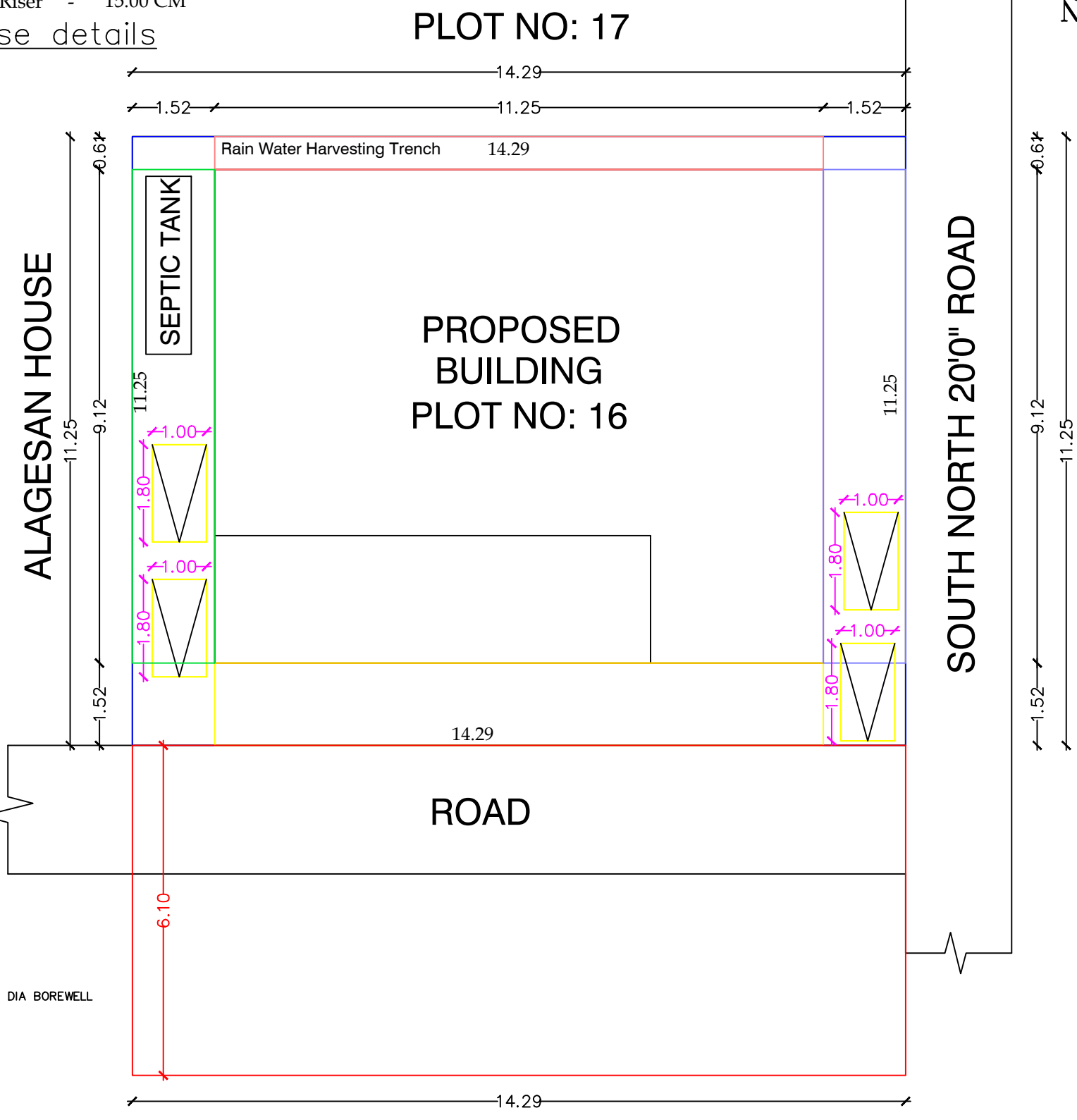
SITE PLAN
