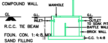
SECTION OF SEP. TANK
