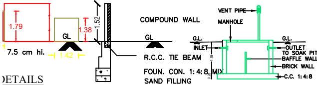
SECTION OF SEP. TANK
