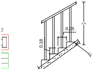
SECTION OF STAIRCASE SCALE 1:100
