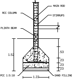
COLUMN DETAILS SCALE 1:100
