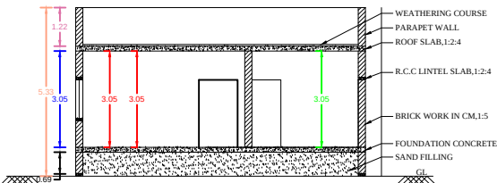
SECTION ON A-A SCALE 1:100
