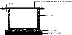
SECTION ON BB SCALE 1:100
