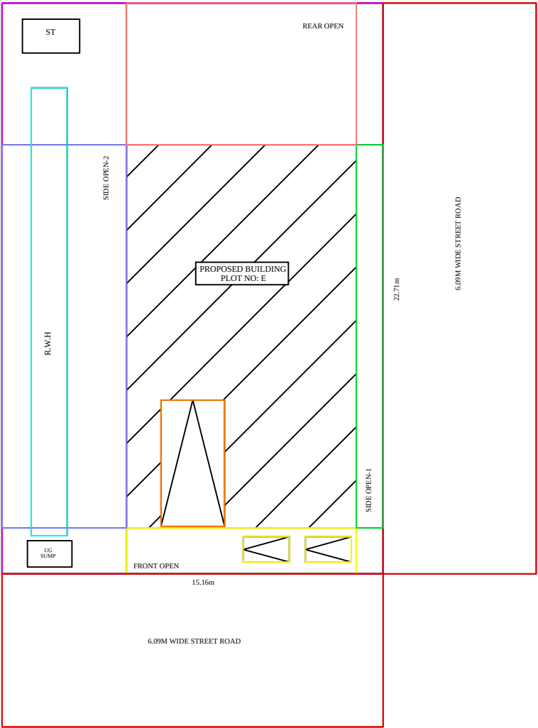
SITE PLAN
