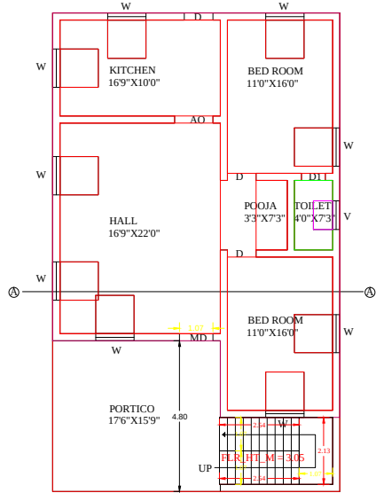
GROUND FLOOR PLAN SCALE 1:100
