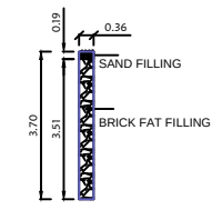
DETAILS OF PERCOLATION PIT
