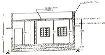
Section on-"AA"
