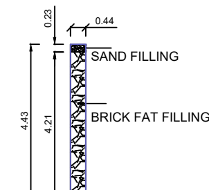
DETAILS OF PERCOLATION PIT
