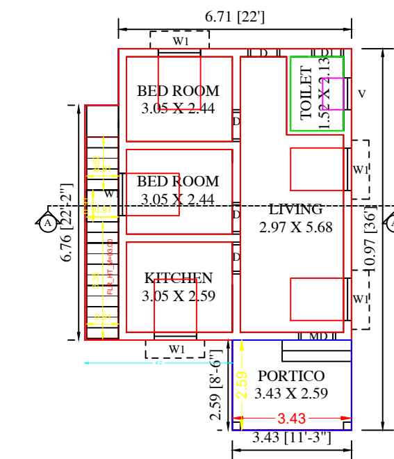
GROUND FLOOR PLAN BLOCK-1
