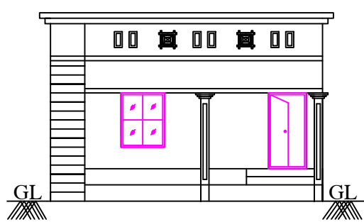
ELEVATION OF BLOCK - 2
