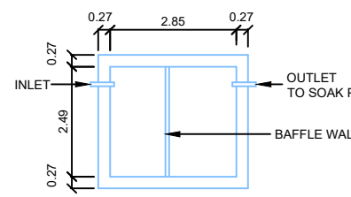
PLAN SEPTIC. TANK
