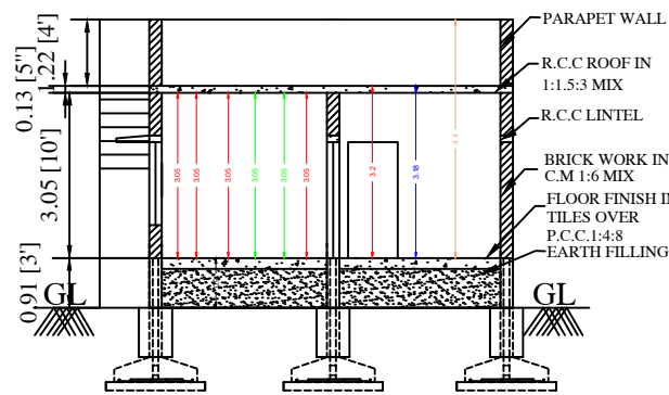
SECTION AA OF BLOCK - 2
