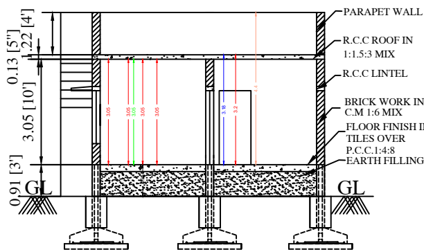
SECTION AA OF BLOCK - 1
