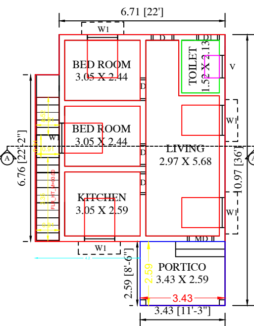
GROUND FLOOR PLAN BLOCK-2
