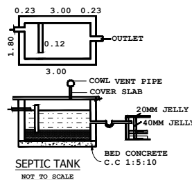
SEPTIC TANK NOT TO SCALE
