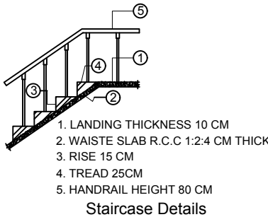
Staircase Details
