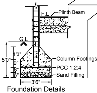
Foundation Details
