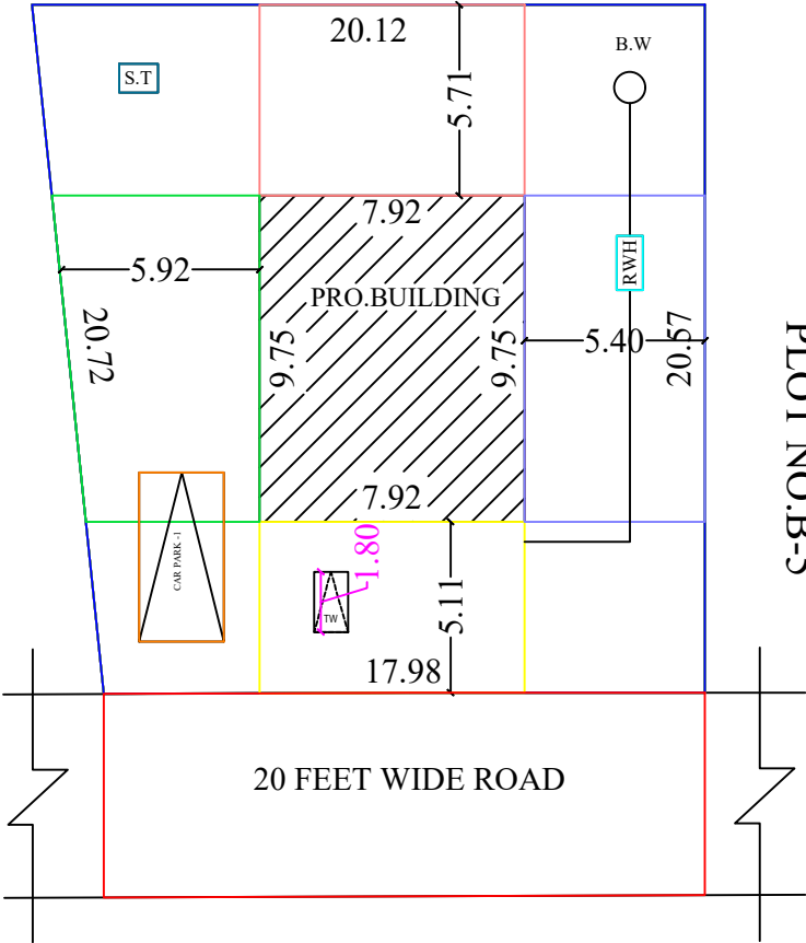
SITE PLAN
