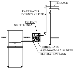
WATER STING SYSTEM
