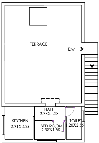
RST FLOOR PLAN
