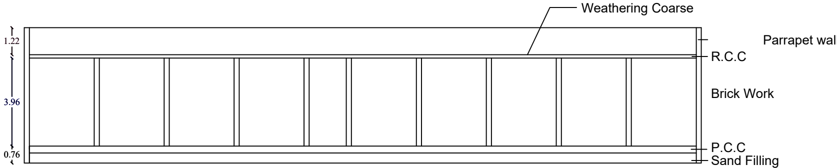
SECTION-A'-A'
