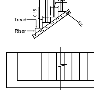
STAIRCASE DETAIL
