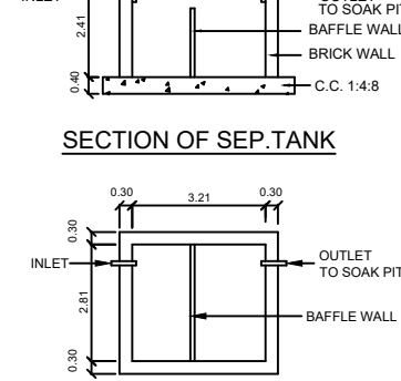
SEPTIC. TANK
