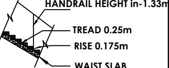
STAIRCASE DETAILS
