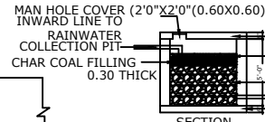
SECTION
