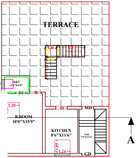
RO.FIRST FLOOR PLAN
