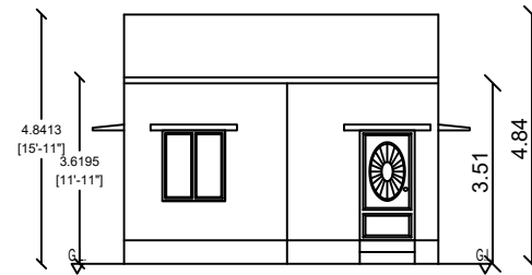
ELEVATION ON EAST
