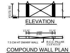
COMPOUND WALL PLAN
