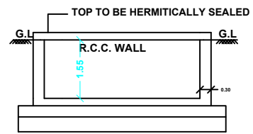
RWHS SECTION (SAMPLE) RWHS_CAPACITY_L = 2000
