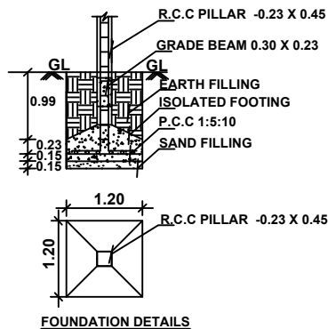
FOUNDATION DETAILS
