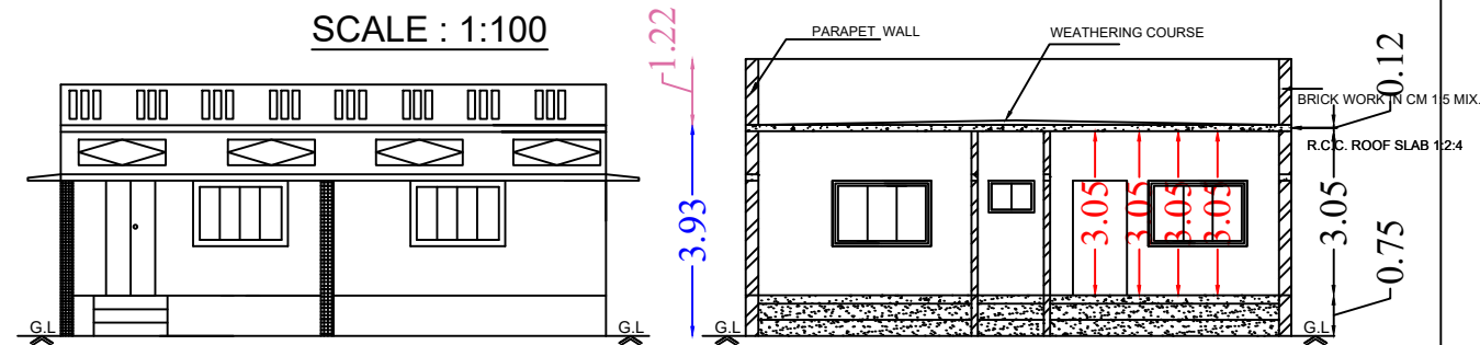
Section on-"AA"
