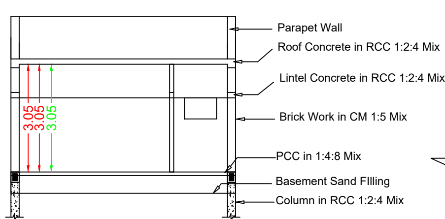
Section RR
