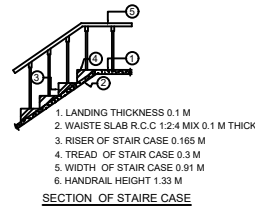
SECTION OF STAIR CASE
