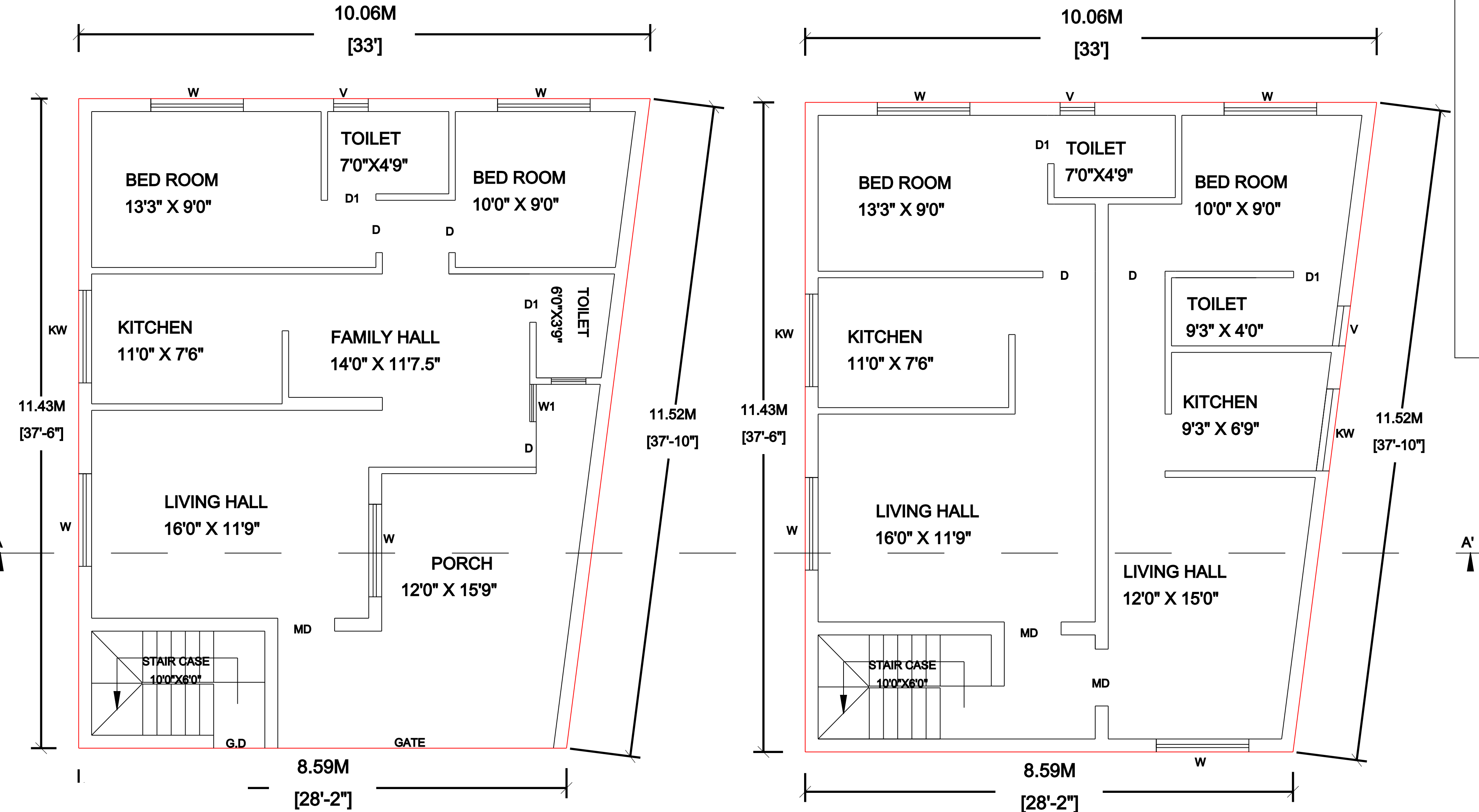
FLOOR PLAN
