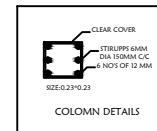
COLUMN DETAILS
