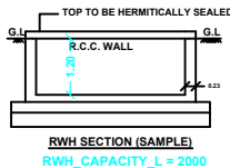
RW SECTION (SAMPLE)
