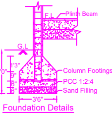
Foundation Details
