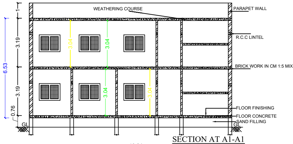
SECTION AT A1-A1
