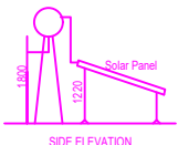
SIDE ELEVATION
