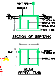
SECTION OF SEPTIC TANK
