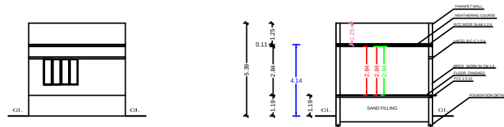
FRONT ELEVATION
