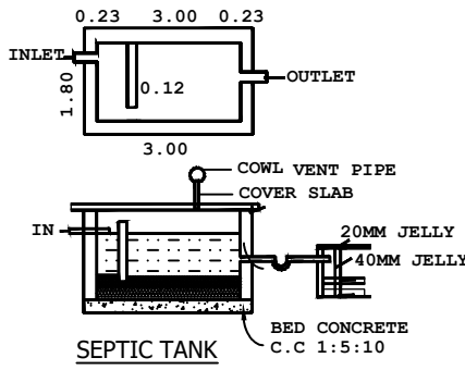
SEPTIC TANK
