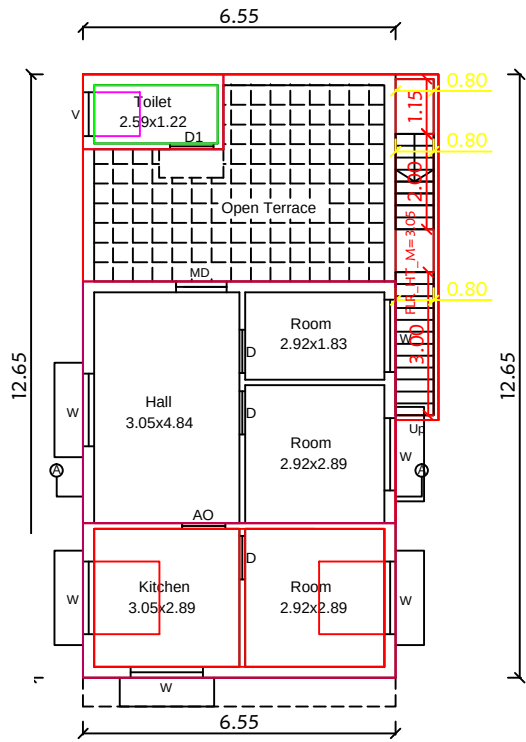
First Floor (Proposed)
