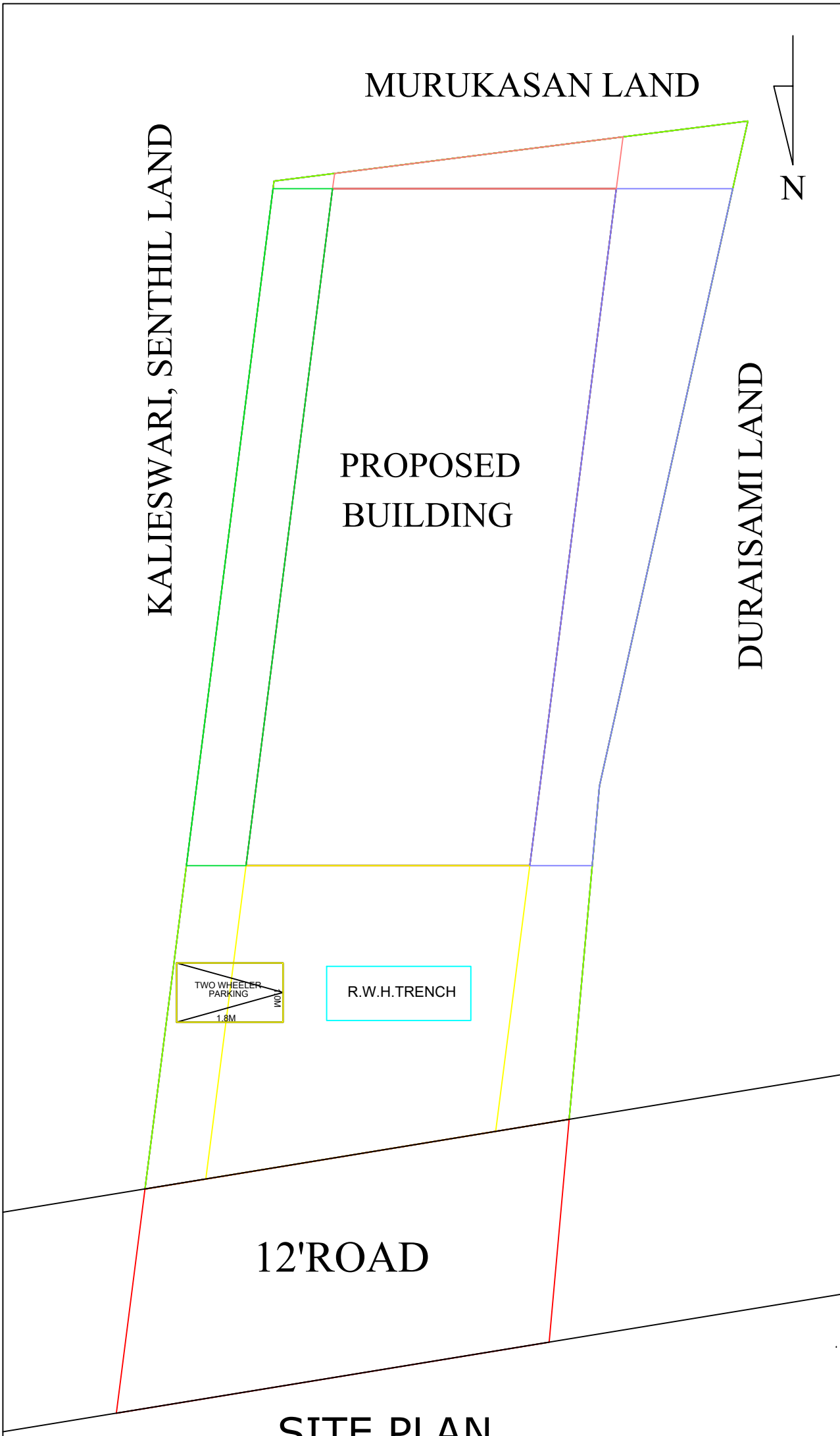
SITE PLAN
