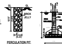
FOUNDATION DETAILS SCALE : 1:50.
