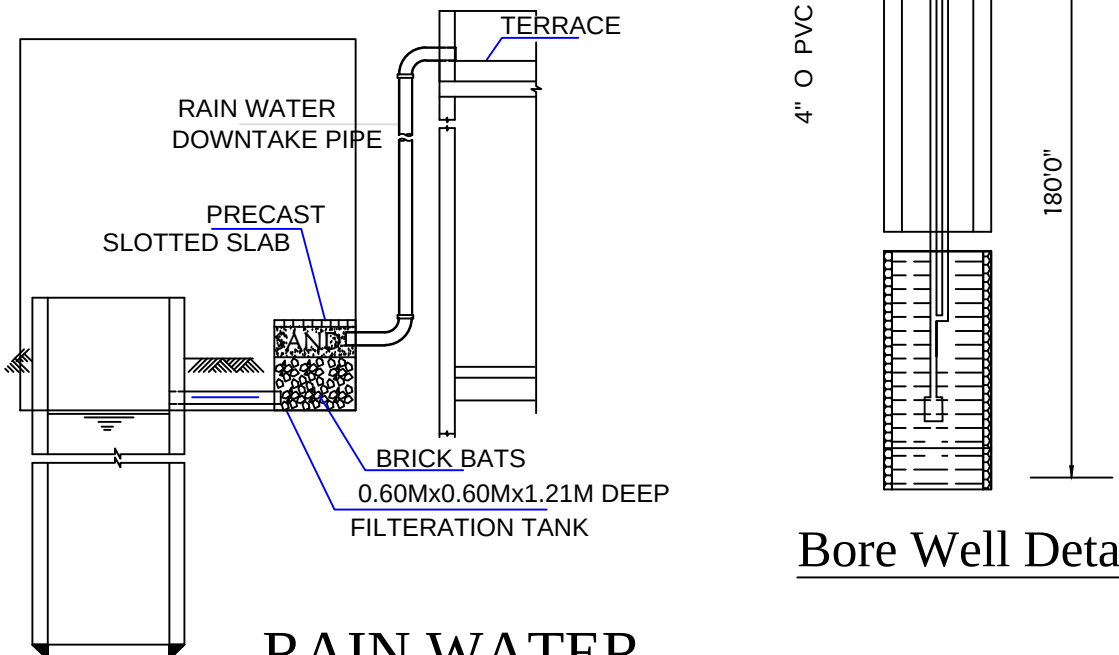
RAIN WATER HARVESTING SYSTEM
