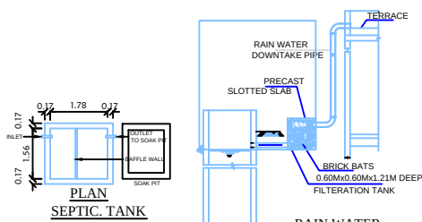
RAIN WATER HARVESTING SYSTEM
