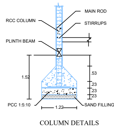
COLUMN DETAILS
