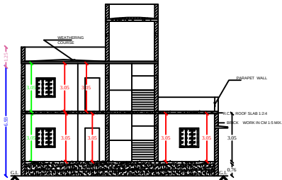
Section on-"AA"
