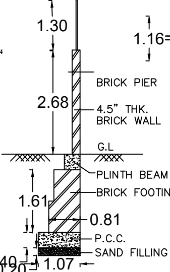
COMPOUND WALL DETAILS
