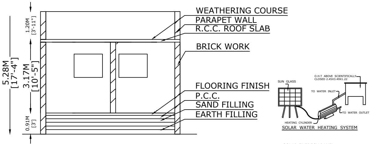
SECTION ON XX
