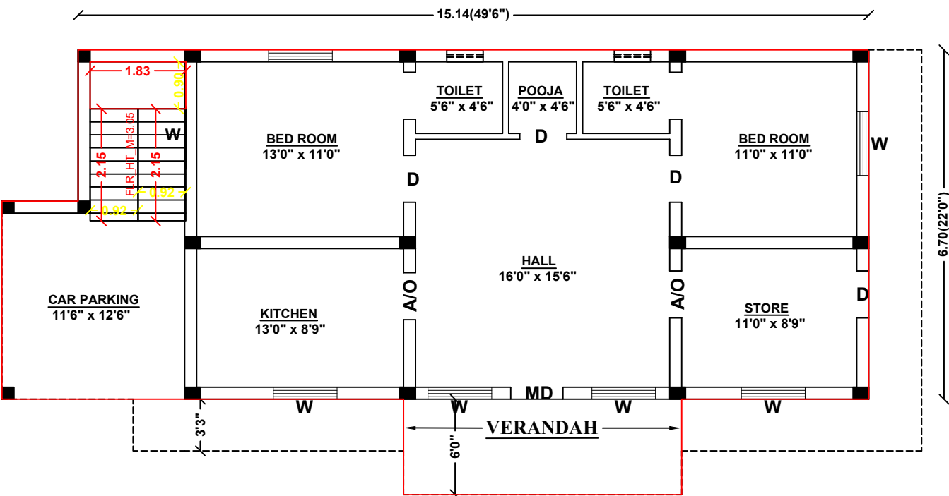
EXT GROUND FLOOR
