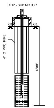
Bore Well Details
