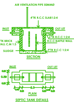
SEPTIC TANK DETAILS
