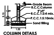
COLUMN DETAILS
