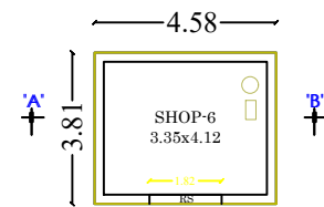
BLOCK II GROUND FLOOR PLAN
