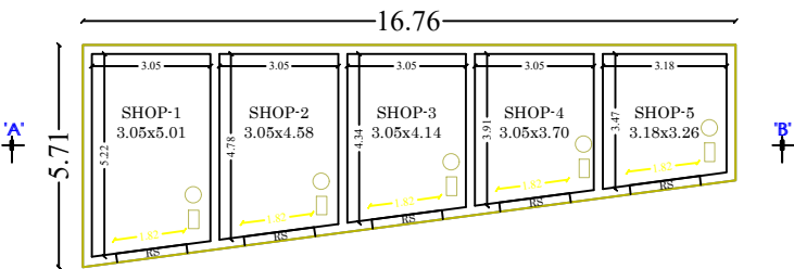
BLOCK I GROUND FLOOR PLAN
