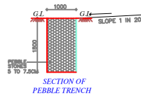
SECTION OF PEBBLE TRENCH
