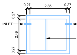
PLAN SEPTIC. TANK
