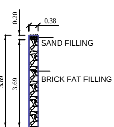
DETAILS OF PERCOLATION PIT
