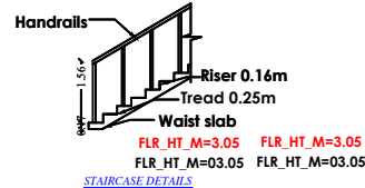
STAIRCASE DETAILS
