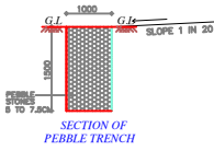
SECTION OF PEBBLE TRENCH
