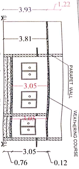
Section on-"AA"
