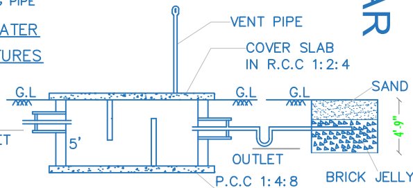
SECTION-AB
